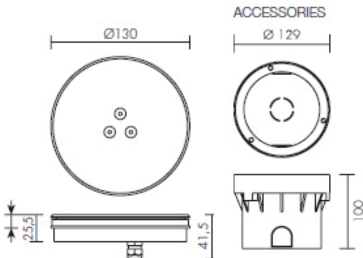
WC0500 Outer casing
